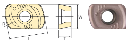
Fig.2: EPMT with Breaker
